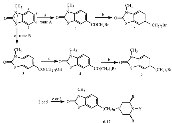
Scheme 1. Synthesis pathway of 6-piperidino or 6-piperazinoalkyl-2(3 H )-benzothiazolones ( 6–17 ). Reagents and conditions: (a) BrCH 2 COCl, AlCl 3 –DMF; (b) Et 3 SiH, TFA; (c) Cl(CH 2 ) 3 COCl, PPA; (d) HBr (gas), acetone, 20 °C; (e) secondary cyclic amine, Et 3 N, acetone reflux, for 24 h; (f) heterocyclic amine, K 2 CO 3 , DMF, for 5 h.
