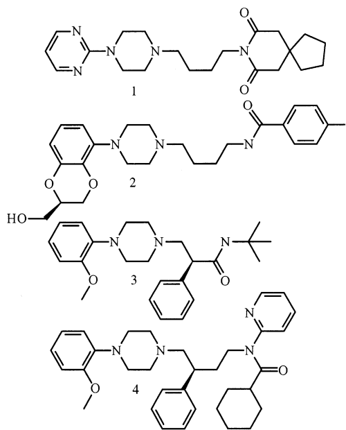
Figure 1. Structure of some 5\text{-HT}_{1A} ligands.
