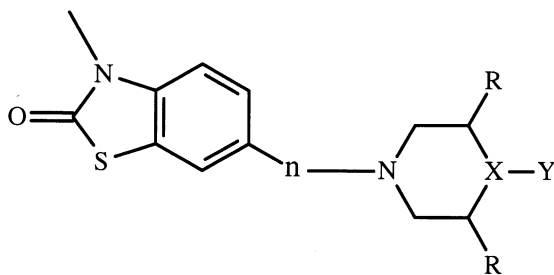
Figure 3. General structure of the mixed sigma/5-HT 1A ligands ( n =number of methylenes, R=H or CH 3 , X=N or CH, Y=phenyl, benzyl, 2,4- or 3,4-dichlorobenzyl).
