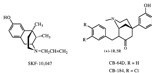
Figure 2. Some examples of sigma 1 and 2 ligands.
